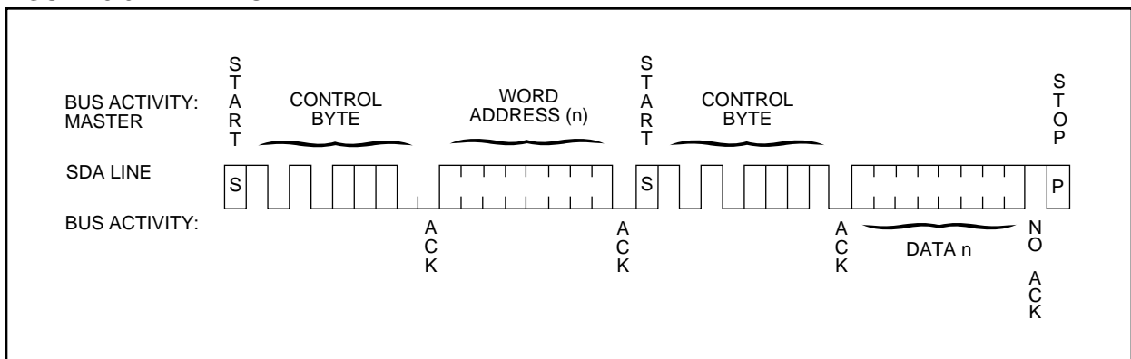
FIGURE 8-3: RANDOM READ
